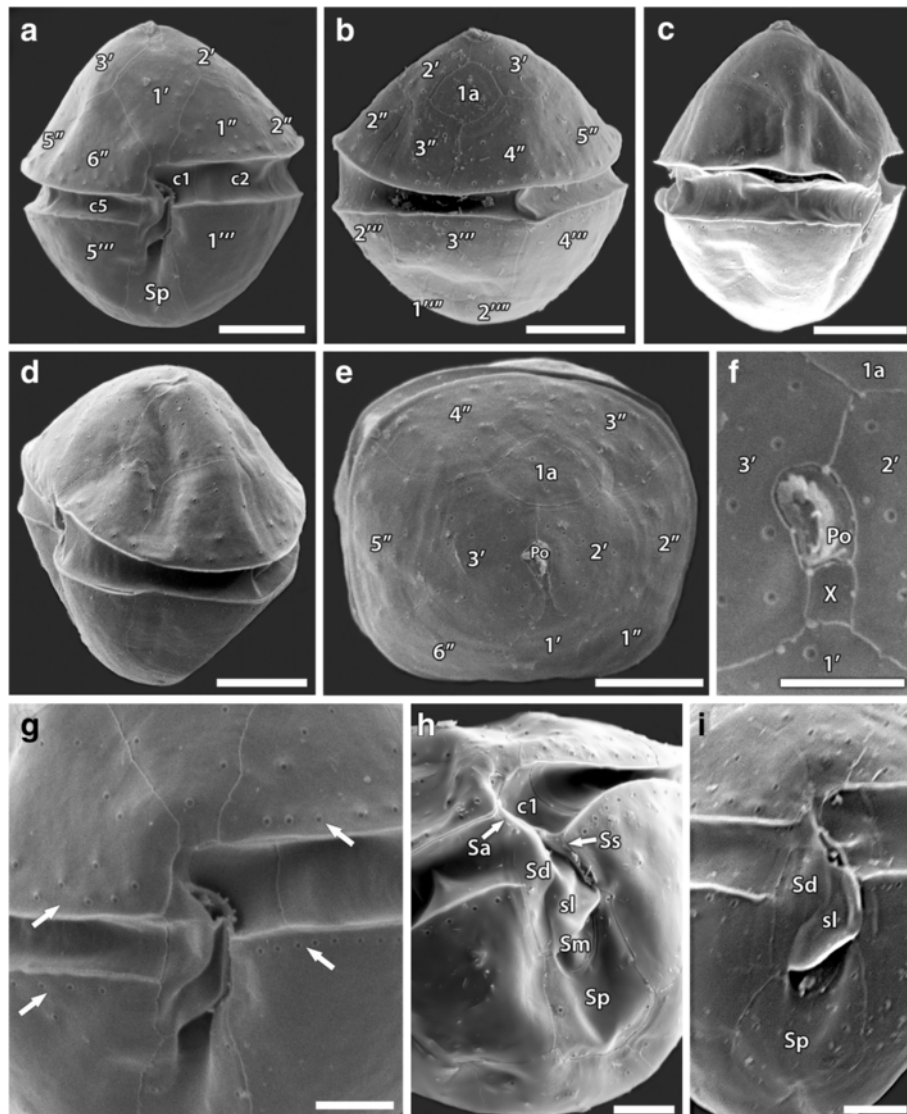
Fig. 3 Scanning electron micrographs of Peridiniopsis minima from Iraq. (a) ventral view; (b) dorsal view; (c) oblique right lateral view; (d) oblique left lateral view; (e) apical view; (f) detail of the apical view showing the apical pore complex with surrounded apical plates; (g–i) detail of theca in ventral view showing marginal rows of densely lying pores (G, arrows) and plate pattern of the sulcal series (h, i). Scale bars: A–E, 5 \mu m; F–I, 2 \mu m
